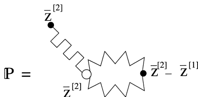
Fig. 4. Diagram \mathbb{P} corresponding to G_A^{*[1]} , G_B^{*[1]} and G_C^{*[1]} after step-2 resummation. The crenelated line is a bond F_{\text{RT}} , while the double wavyline corresponds to a bond (1/2)[F^{\text{cc}}]^2 . The rule \mathcal{R}_2 is illustrated in the present example.
