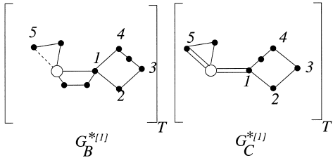
Fig. 3. Step-2 for resummations. G_B^{*[1]} and G_C^{*[1]} are two G^{*[1]} diagrams which correspond to the same prototype diagram \mathbb{P} as the diagram G_A^{*[1]} in Fig. 2. The brackets with an index T indicate that the diagrams G^{*[1]} must be calculated with the weights and the subtraction (rule \mathcal{R} ) displayed in Fig. 2.
