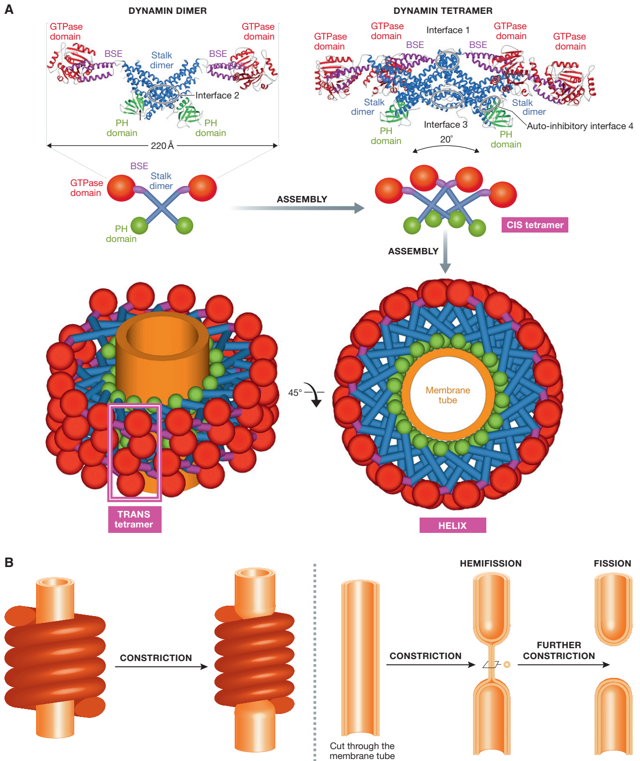
Figure 1. Structure and assembly of dynamin.
