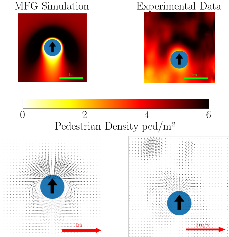
Figure 4.11: Qualitative comparison between density, first row, and velocity plots, second row, between the experiment, right column, and the ergodic state of the MFG model, with parameters \xi = 0.4 , c_s = 0.2 and \gamma = 6 , left column, for the case where pedestrians were giving their back to the incoming cylinder and were asked not to anticipate. Image taken from [16].
