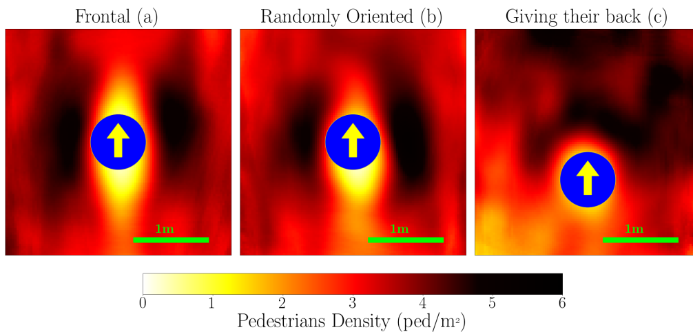
Figure 1: Experimental results of the passage of a cylindrical intruder (blue disc) through a static dense crowd for an average density of \sim 3.5 \text{ ped/m}^2 for three different configurations. In (a) pedestrians were all facing the obstacle, in (b) they were randomly oriented and in (c) participants were asked to give their back to it and not to anticipate. Data from [7].
