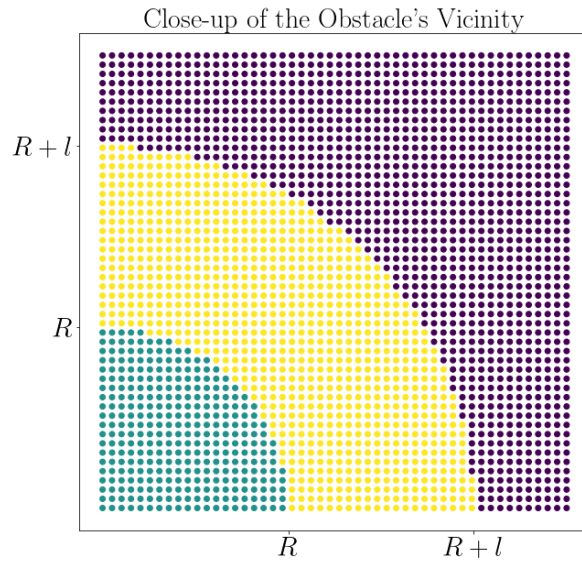
Figure 4.12: Sketch of the close-up of the grid \mathcal{G} in the vicinity of the cylinder. The green points represents the cylinder. The yellow points are where we solve the MFG equations in the (\Phi, \Gamma) formulation, whereas for the purple points we solve them in the (u, m) one. Although in the picture the yellow area seems large with respect to the green one, in the real implementation, since l is small with respect to the cylinder's radius, the yellow area would be much thinner.
