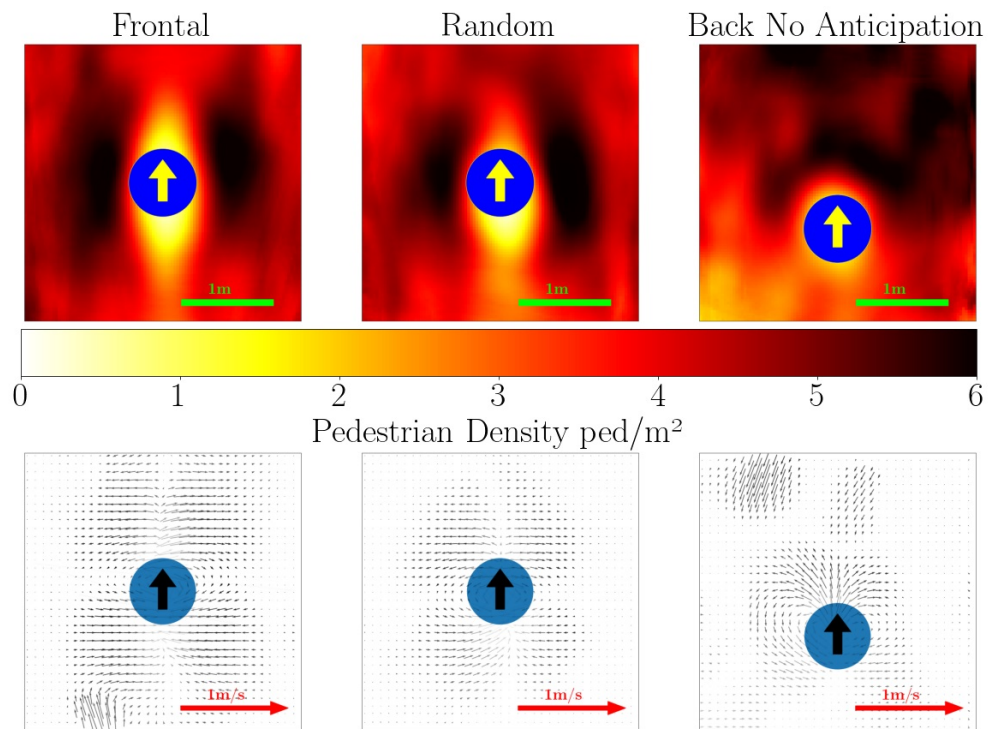
Figure 4.1: Experimental results of the passage of a cylindrical intruder (blue disc) through a static dense crowd for an average density of \sim 3.5 \text{ ped/m}^2 for the three different configurations of the experiment of section 1.2. Top row: densities plots. Bottom row: velocity fields. Data from [75]. Figures extracted from [16].
