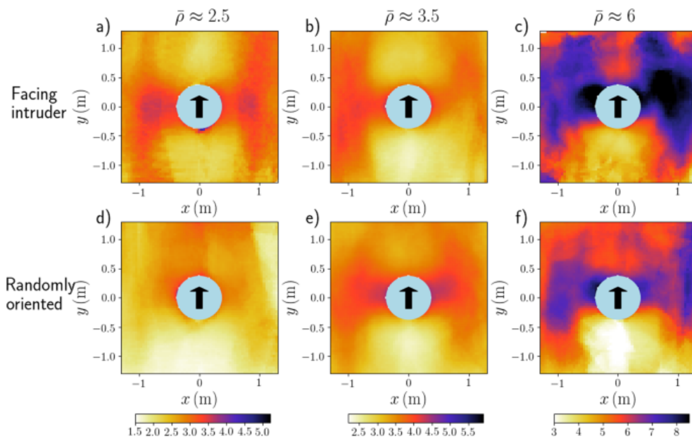
Figure 1.4: Top row: density plots with averages 2.5\text{ped}/\text{m}^2 , 3.5\text{ped}/\text{m}^2 and 6\text{ped}/\text{m}^2 for the experimental configuration where participants were all facing the intruder. Bottom row: same as top row, but for the configuration where pedestrians were randomly oriented. Image taken from [75].
