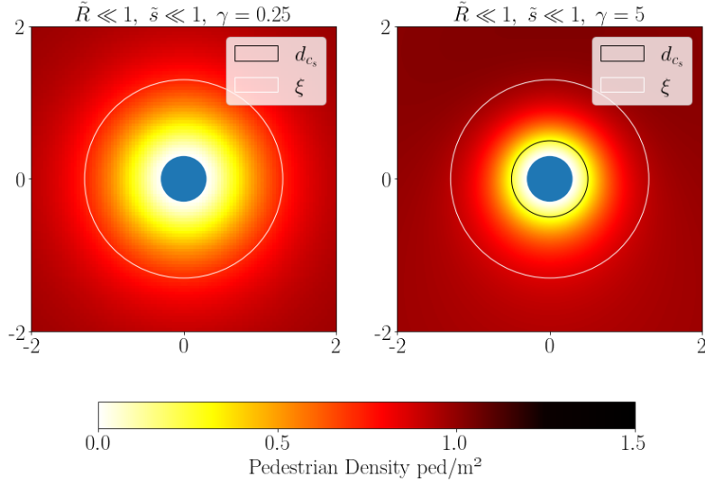
Figure 4.8: Focus on the quadrant III of Figure 4.7 with details about the size of the perturbation. The white circle has radius R + \xi whereas the black circle has radius R + d_{cs} , with d_{cs} \equiv c_s/\gamma (note that the left panel's black circle is not visible since d_{cs} = 4 ). We observe how the smallest of the circles is the one governing the distance at which the perturbation due to the cylinder is felt. Image taken from [16].
