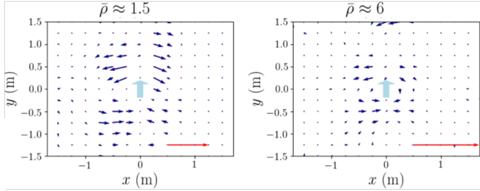
Figure 1.5: Experimental velocity field obtained with the configuration where pedestrians were all facing the incoming intruder. Regardless of the average density ( 1.5\text{ped}/\text{m}^2 on the left, 6\text{ped}/\text{m}^2 on the right) we observe a clear anticipation pattern with pedestrians moving laterally well in advance. Image taken from [75].
