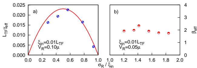
Figure 2: (color online) a) Lyapunov exponent \gamma_{\text{eff}} in units of 1/L_{\text{TF}} for the localized BEC in a speckle potential, in the regime \xi_{\text{in}} > \sigma_{\text{R}} . The solid line is \gamma(1/\xi_{\text{in}}) from Eq. (13). b) Exponent of the power-law decay of the localized BEC in the regime \xi_{\text{in}} < \sigma_{\text{R}} . The parameters are indicated in the figure.
