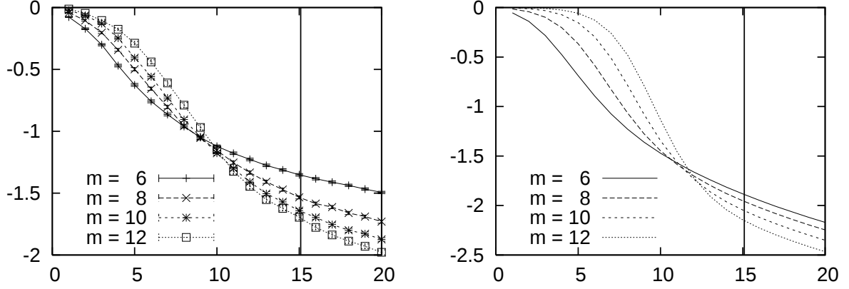
FIG. 4: The overlap q_{typ} as a function of \ell at T = 0.8 . Left panel: numerical values obtained through the transfer matrix algorithm for various values of m . Right panel: analytic curves obtained through the approximations discussed in the text. The vertical lines marks the value of \ell_c in the m \rightarrow \infty limit.
