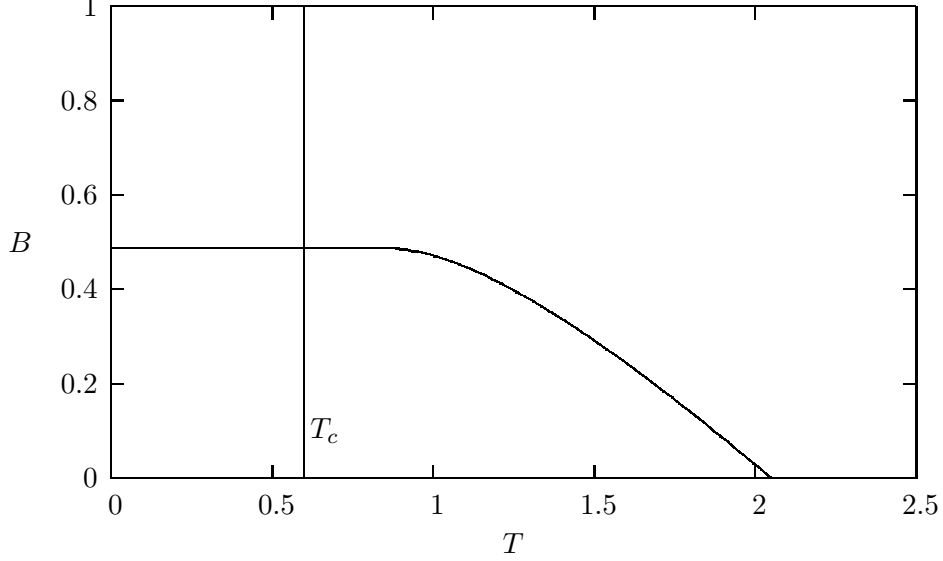
FIG. 2: The free-energy barrier to relax from the ground state \vec{\sigma}^* .
