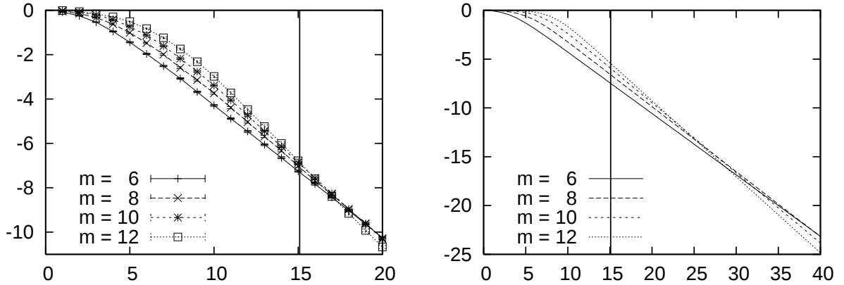
FIG. 5: Same as figure 4 for the quantity p_{typ} .
