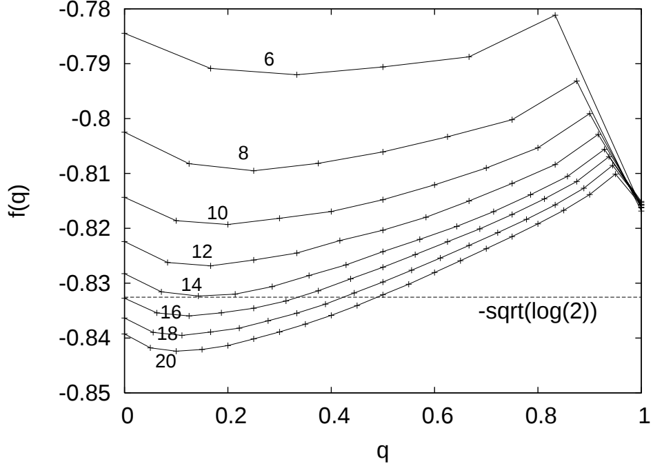
FIG. 7: Window free-energy for T = 0.8 , m = 12 and many different values of \ell , from 6 (top) to 20 (bottom).
