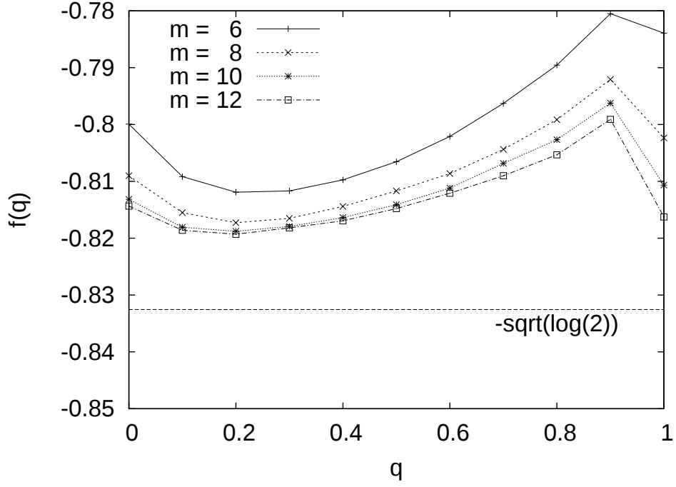
FIG. 6: Window free-energy for \ell = 10 and T = 0.8 as a function of the overlap with respect to the ground state configuration.
