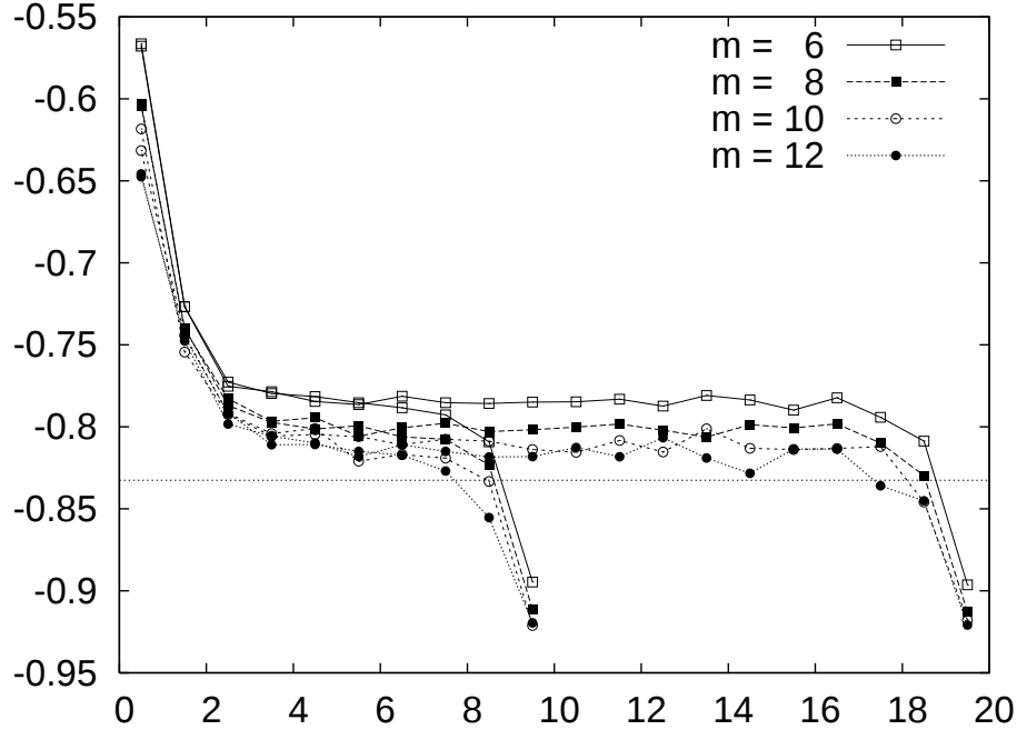
FIG. 3: The mean value of the ground state link energy as a function of the position in the system for L = 10 and L = 20 . On the left boundary the configuration is fixed, while on the right end the system is free. The horizontal line is -\sqrt{\log(2)} .
