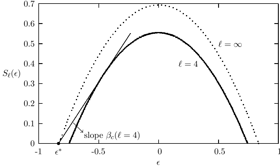
FIG. 1: Microcanonical entropy for the full system ( \ell = \infty , dotted line) and for a window of size \ell = 4 (thick line). A system prepared in the ground state of the full system (big dot) and constrained in a window of size \ell = 4 makes a first order transition at inverse temperature \beta_c(\ell = 4) (the slope of the thin line).
