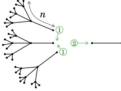
Figure 3: Cayley tree of coordination number z (here 4) and depth n (here 3 before attachement and 4 after).
