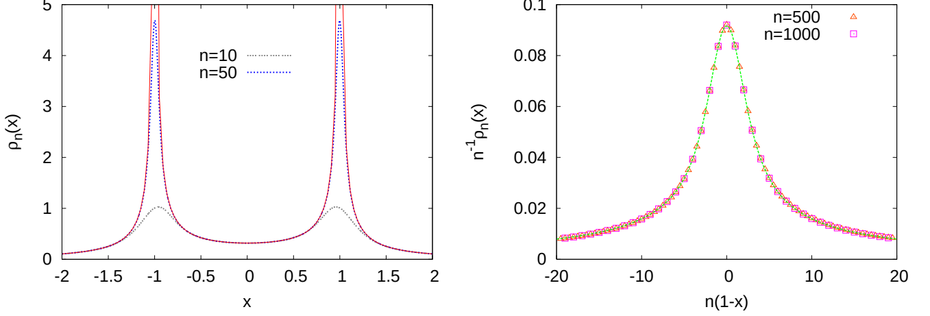
FIG. 1: Left : Mean density of real roots \rho_n(x) for Kac polynomials K_n(x) (3) and d = 2 as a function of x for different values of n = 10, 50 (dotted lines). The solid line is the analytic expression \rho_\infty(x) in Eq. (25) for |x| < 1 and in Eq. (27) for |x| > 1 . Right : Plot of n^{-1}\rho_n(x) as a function of n(1-x) for n = 500, 1000 (and thus x close to \pm 1 ). The dotted line is the function \rho^K(y) in Eq. (31). There is no fitting parameter.
