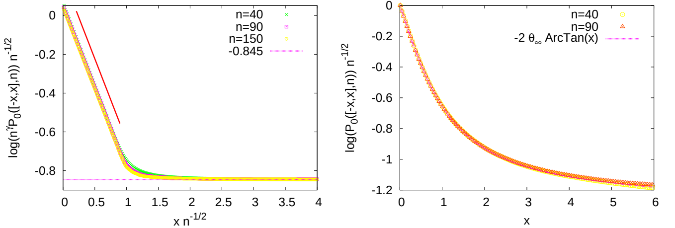
FIG. 7: Left : Plot of [\log(n^\gamma P_0([-x, x], n))] n^{-1/2} for Weyl polynomials W_n(x) (6) as a function of x/\sqrt{n} for different values of n = 40, 90 and 150 . Here \gamma = 0.10(1) and the solid line has slope -0.845 . Right : Plot of [\log P_0([-x, x], n)] n^{-1/2} for binomial polynomials B_n(x) (7) as a function of x for different values of n = 40 and 90 . The solid line is the exact result in Eq. (94) with \theta_\infty = 0.42(1) , which is the only fitting parameter here.
