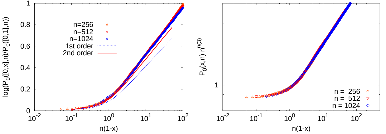
FIG. 4: Left : Plot of \log[P_0([0, x], n)/P_0([0, 1], n)] for Kac polynomials K_n(x) and d = 2 as a function of n(1-x) for different degrees n = 256, 512, 1024 . The dotted line is the result of the Mean Field prediction (73) and the solid line the result of the second order calculation in the \epsilon expansion (83). Right : Plot of n^{\theta(3)} P_0([0, x], n) on a log-log scale for Kac polynomials K_n(x) and d = 3 with \theta(3) = 0.238(4) as a function of n(1-x) for different degrees n = 256, 512, 1024 .
