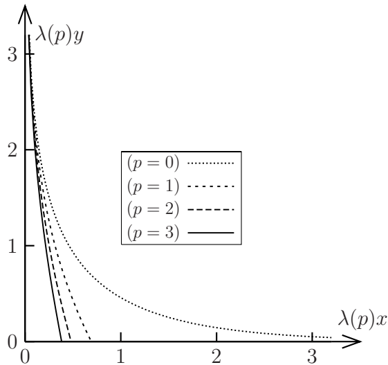
Figure 2: Limit shapes for the minimal difference p partitions with p = 0, 1, 2 , and 3 , where \lambda(0) = \pi/\sqrt{6} , \lambda(1) = \pi/\sqrt{12} , \lambda(2) = \pi/\sqrt{15} , and \lambda(3) = 0.752617\dots
