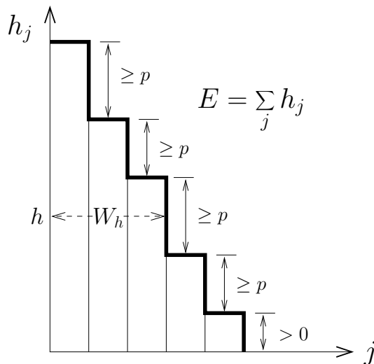
Figure 1: A typical Young diagram for MDP- p problem. The thick solid border shows the height profile or the outer perimeter. W_h is the width of the Young diagram at a height h , i.e., W_h is the number of columns whose heights \geq h .
