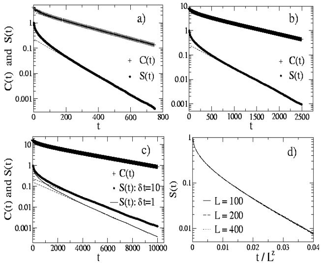
FIG. 1: S(t) and C(t) for the Langevin equation of Eq.(1). The dashed lines are fits of the long-time data to an exponential form. In panels (a-c), the uppermost plots show the data for C(t) . Panel (a): L = 100 , \delta t = 0.625 . Panel (b): L = 200 , \delta t = 2.5 . Panel (c): L = 400 , \delta t = 10.0 (upper plot) and \delta t = 1.0 (lower plot). Panel (d): Finite-size scaling of S(t, L, \delta t) . Results for S for 3 different sample sizes with the same value of \delta t/L^z ( z = 2 ) are plotted versus t/L^z .
