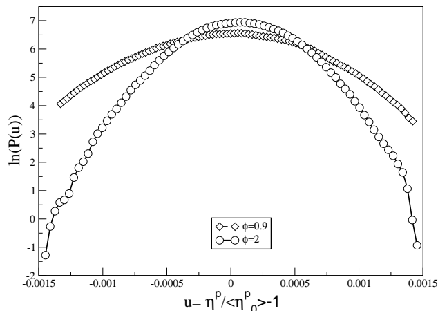
FIG. 8: Linear-log plot of the aggregate size distribution for p = 3/2 and two reduced volume fractions ( \phi^* = 0.9 and 2 ). The data are obtained following over time the different sizes taken by the (unique) condensate. Here, P denotes the probability distribution function of y = \eta^p / \langle \eta_0^p \rangle - 1 .
