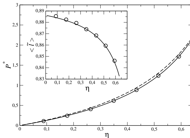
FIG. 6: Equation of state as a function of line coverage \eta when p = 2 , in which case the critical line coverage \eta_c = 2/3 corresponds to \phi_c^* = \sqrt{2/3} \simeq 0.816 . The exact pressure is shown by the continuous line, while the dotted curve is for the crude approximation where \langle \tilde{\ell} \rangle is assumed density independent and equal to its critical value \sqrt{2/3} , which leads to P^* = \sqrt{3/2}\eta/(1-\eta) . Circles : Monte Carlo results with N = 1000 . The inset shows the density dependence of \langle \tilde{\ell} \rangle .
