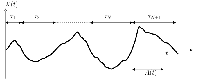
FIG. 1: Intervals between zero-crossings (excursions) of a stochastic process X(t) .
