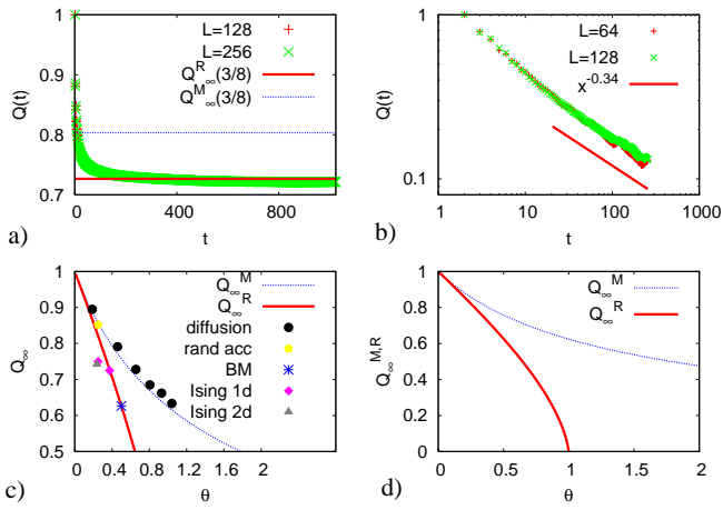
FIG. 2: a) : Q(t) as a function of t for the local magnetization in the Ising chain evolving with Glauber dynamics at T = 0 . b) : Q(t) as a function of t on a log-log scale for the magnetization of a line in the 2d -Ising model at T_c evolving with Glauber dynamics starting from a fully magnetized state. c) : Q_\infty as a function of \theta : the lines correspond respectively to Q_\infty^R(\theta) (solid) and Q_\infty^M(\theta) (dotted) and the points correspond to the numerical values obtained for different nonequilibrium systems. The two values for ‘Ising 1d’ correspond to the local magnetization ( \theta = 3/8 ) and to the global one ( \theta = 1/4 ). d) : Same plot as in c) on a larger scale.
