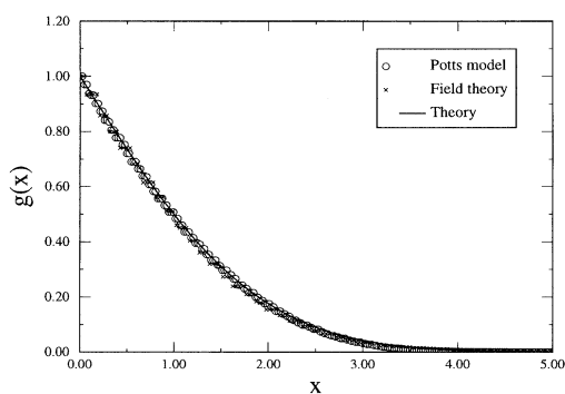
FIG. 1. Comparison of the scaled equal-time correlation functions generated by numerical simulation of the Potts model with q = \infty (in fact q equals the initial number of bubbles \sim 32000 ), numerical integration of Eq. (3) with q = 50 , and the large q analytical result.
